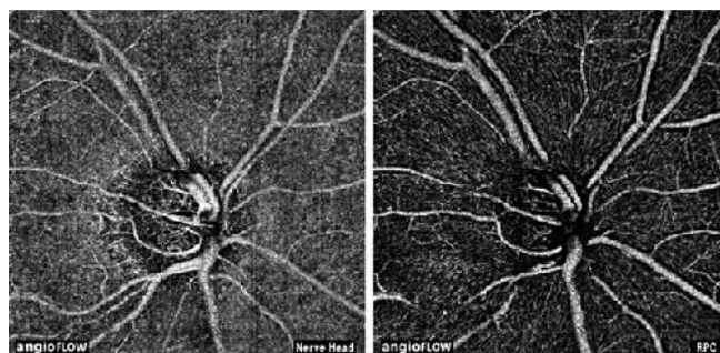
Fig. 5 | Optical coherence tomography angiography (OCTA) of a healthy subject showing a dense vascular network inside and around the optic disc.
