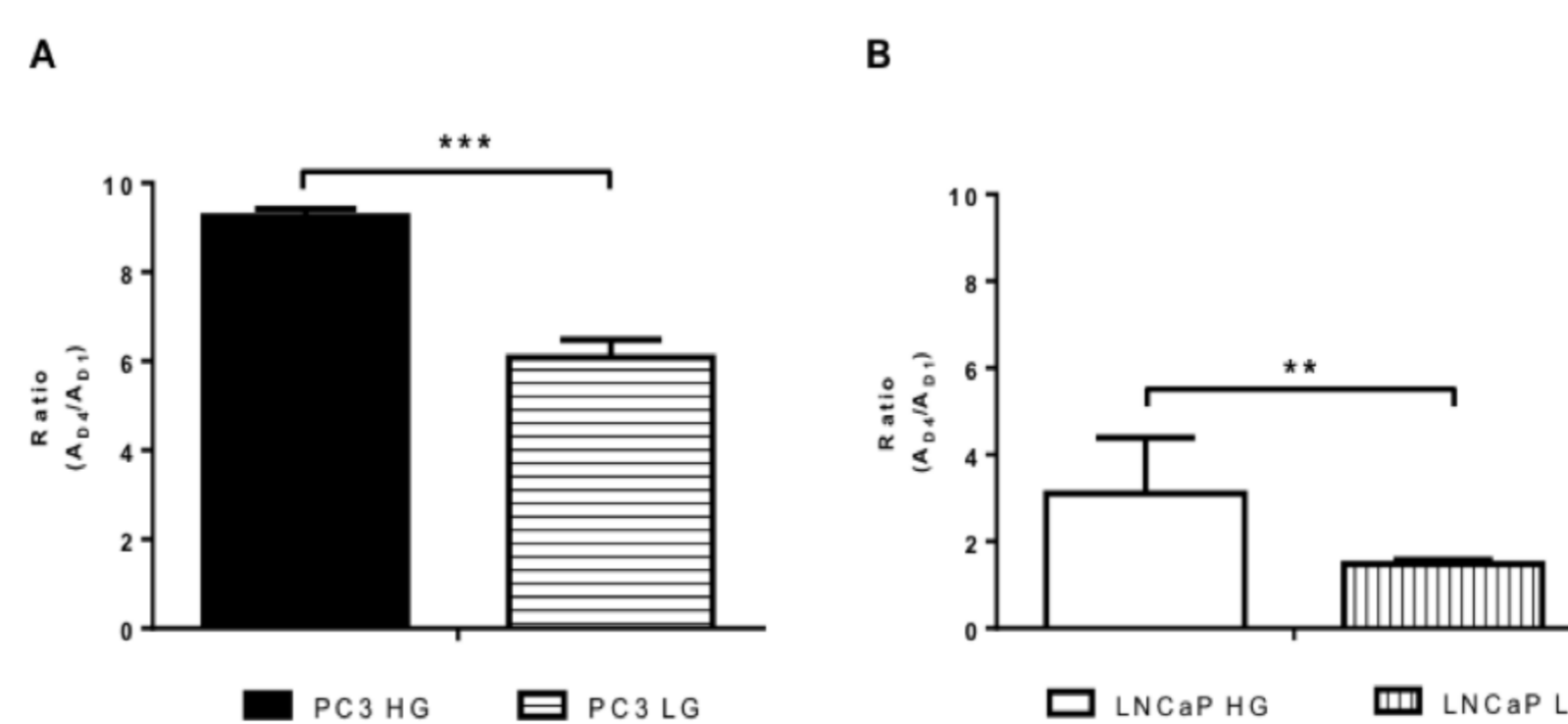
Figure 3 - Results represent the ratio between the measured absorbance after 96h (day 4, A_{96} ) and after 24h (day 1, A_{24} ) for PC3 (A) and LNCaP (B). Results were obtained with six independent experiments. Values represent mean±SEM. Statistical significance: ** p < 0.01 ; *** p < 0.001
