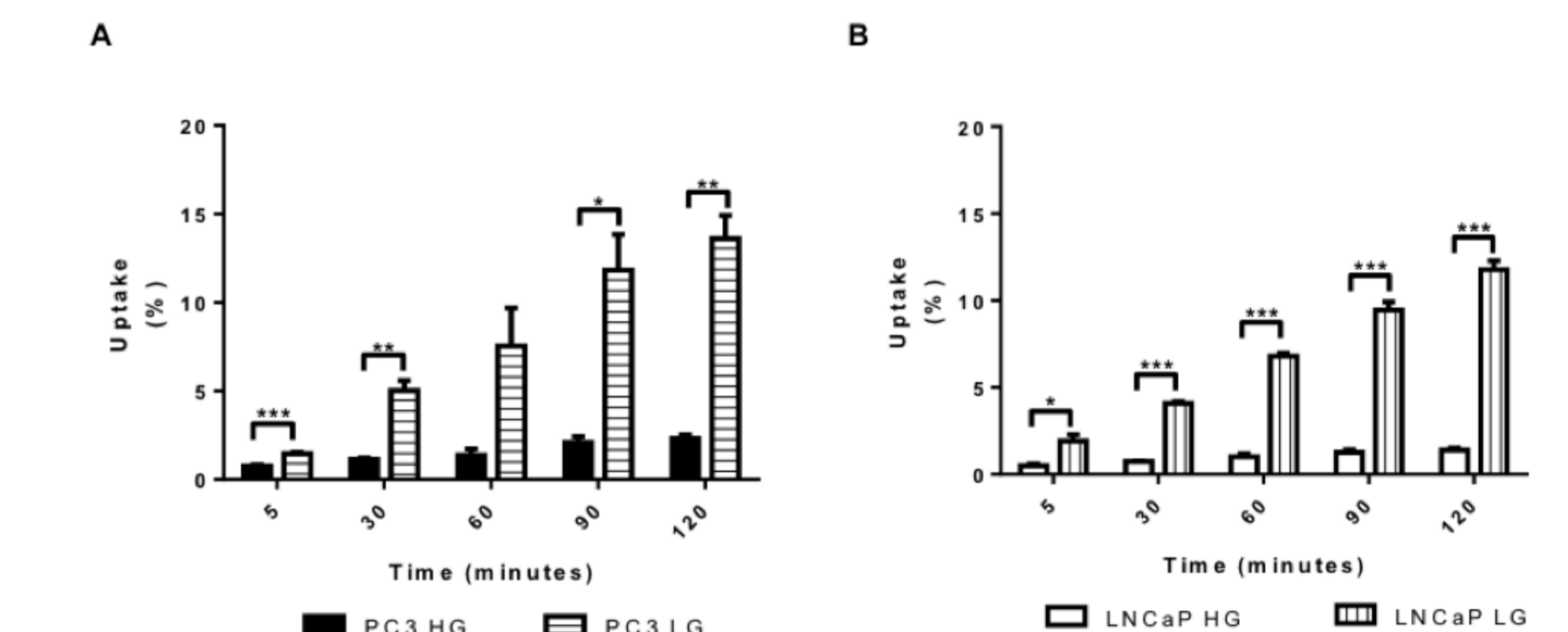
Figure 4 - ^{18}\text{F} -FDG uptake in PC3 (A) and LNCaP (B) prostate cancer cells cultures in high and low glucose media, expressed as percentage of uptake. Results are presented as mean±standard error of a minimum of four independent experiments. Statistical significance: * p < 0.05 ; ** p < 0.01 ; *** p < 0.001 .
