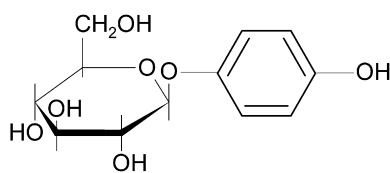
Fig. 1. Chemical structure of arbutin (4-hydroxyphenyl- \beta -D-glucopyranoside).
